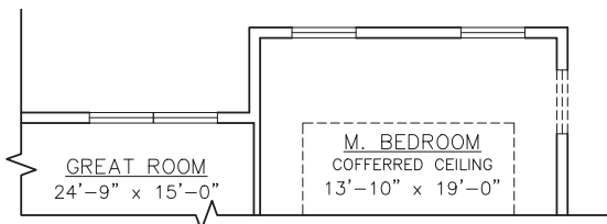
OPT. 4' MASTER BEDROOM EXTENSION
