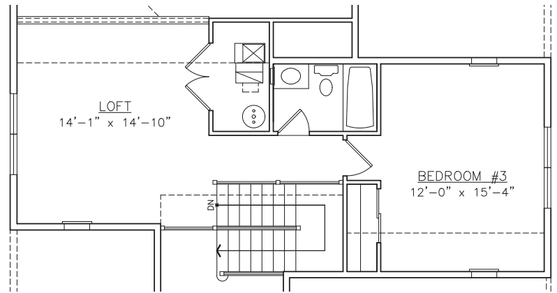
LOFT W/ BEDROOM #3 & BATH PLAN
