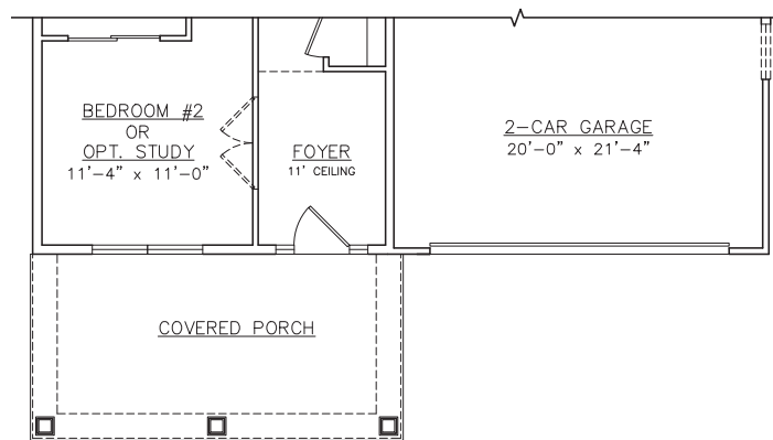
FIRST FLOOR PLAN - OPT. 4' PORCH EXTENSION
