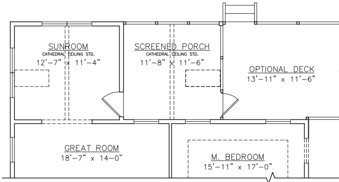
OPT. DECK W/ SUNROOM / SCREENED PORCH
