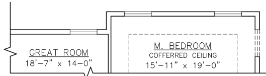
OPT. 2' MASTER BEDROOM EXTENSION
