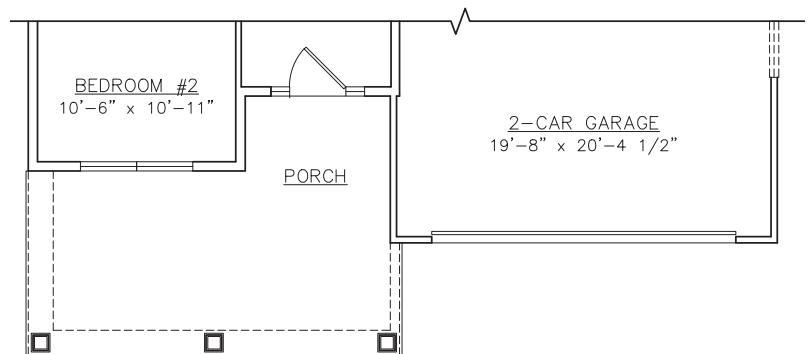
FIRST FLOOR PLAN - OPT. 4' PORCH EXTENSION
