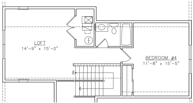
LOFT W/ BEDROOM #4 & BATH PLAN
